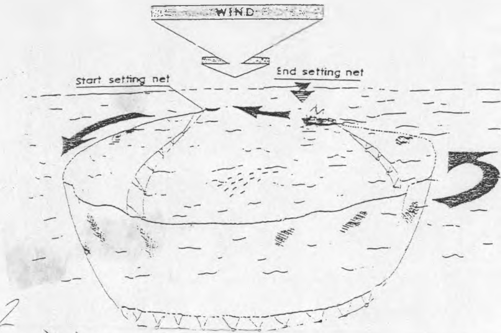
Fig. 9.14 Surrounding a fish school with due regard to wind direction.
