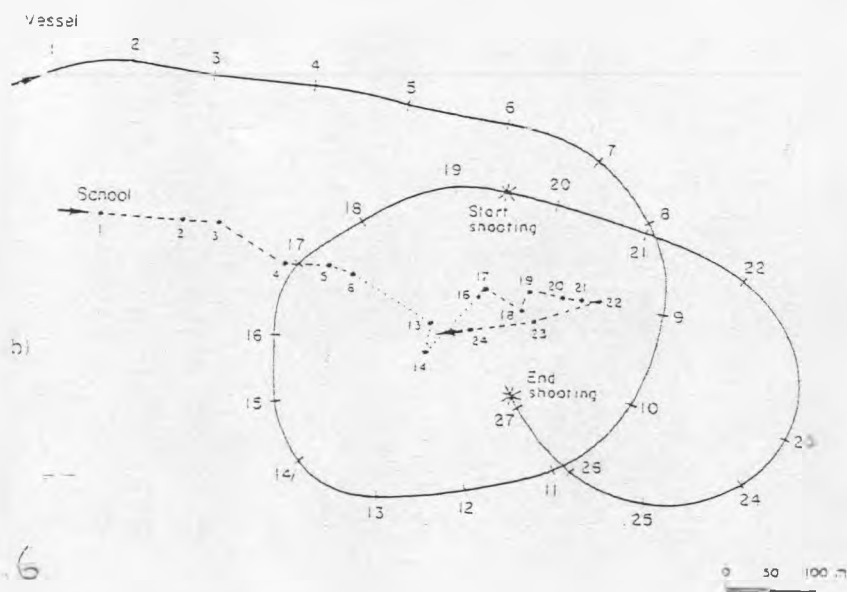
Fig. 9.18 Horizontal movement of mackerel schools in purse seine capture situations (after Misund 1987).
